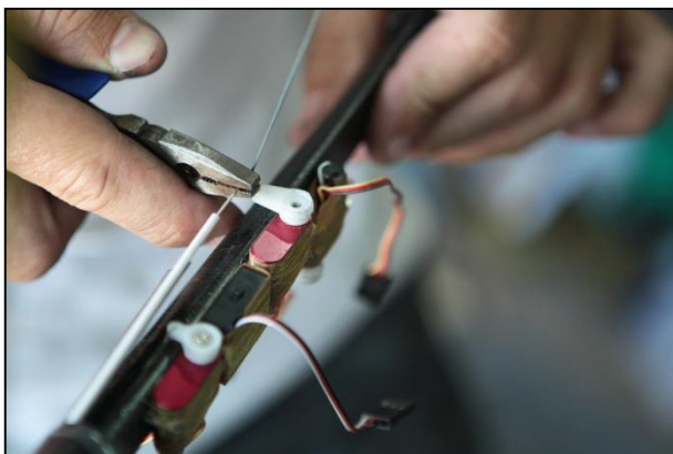
Figure 2.37 - Link aileron
