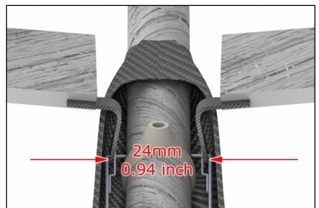
2.24 - The distance between the flaperon horns
