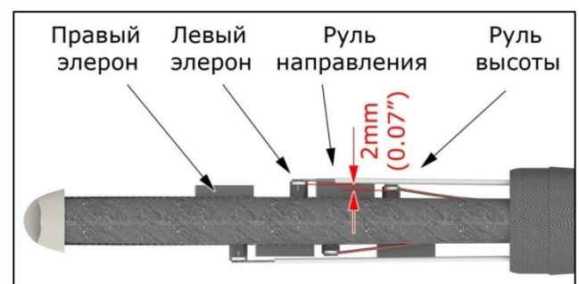
Figure 2.26 - Placement of equipment in the nose Snipe
